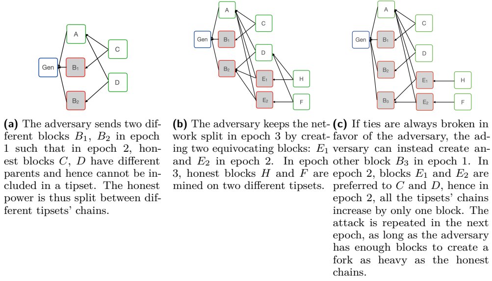
■ Figure 3 n -split attack. Each block filled in grey is an equivocating block, meaning they were created by the adversary using the same leader election proof in one epoch. Each green block is an honest block.
